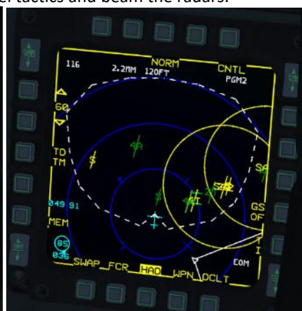
PGM2
