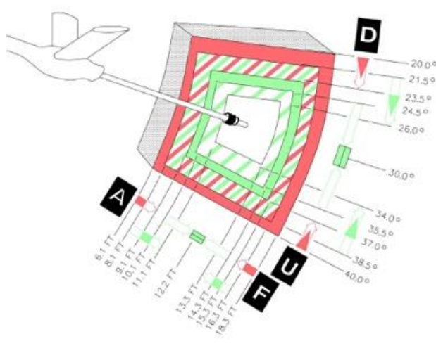
Director lights envelope of the KC-135
